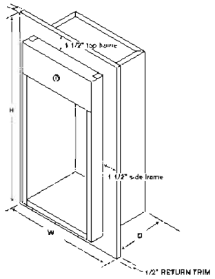
SEMI-RECESSED 999-SR (10 LB) ROUGH OPENING DIMENSIONS
